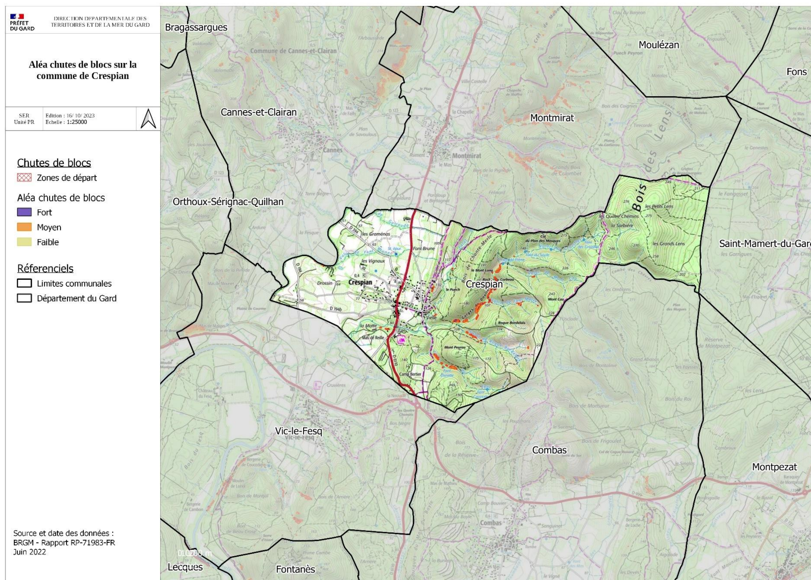
Figure 69. Aléa Chutes de blocs
